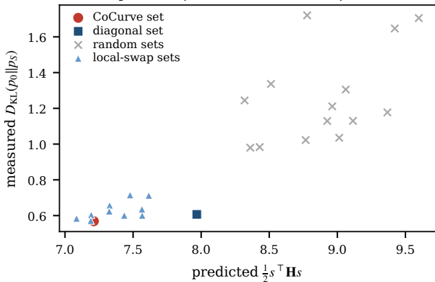
Same-budget discrimination Spearman \rho=0.87 over 26 sets at \rho=20\%
